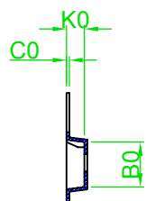
B-B' Section
