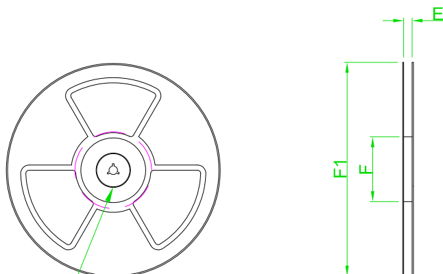
Detail C SCALE 1: 8
