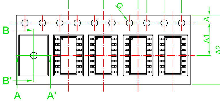
B-B' Section
