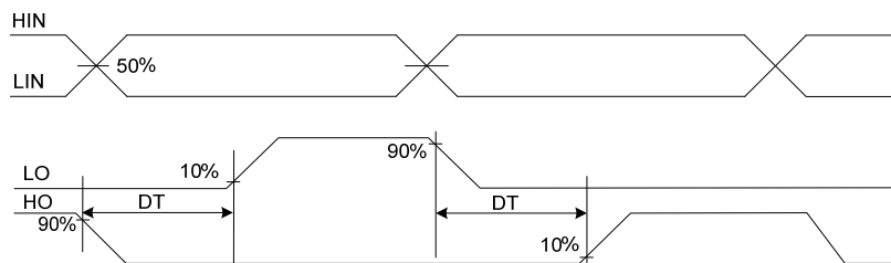
INTERANL DEADTIME TIMING
